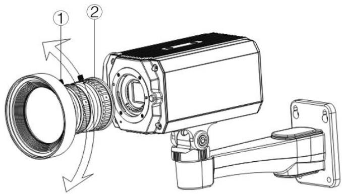
Figure 8-3 Lens installation (2)
